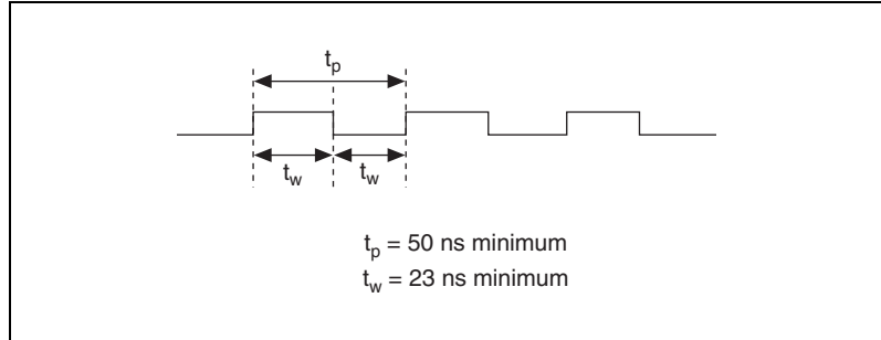
Figure 5-10. MasterTimebase Timing Requirements
